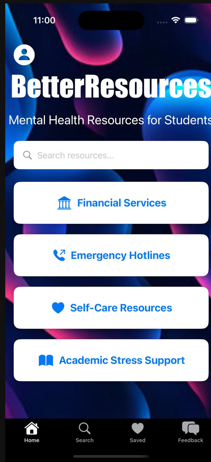
Home Page
